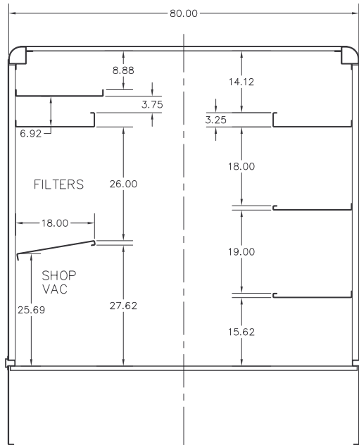
CROSS SECTION BAY #1
